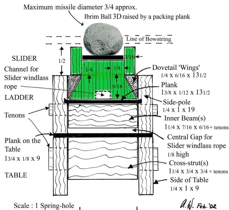
Figure 4. Cross-section of ballista stock from Vitruvius' description, with ovoid Ibrim Ball 3D raised by a packing plank. See Section 5 text.
